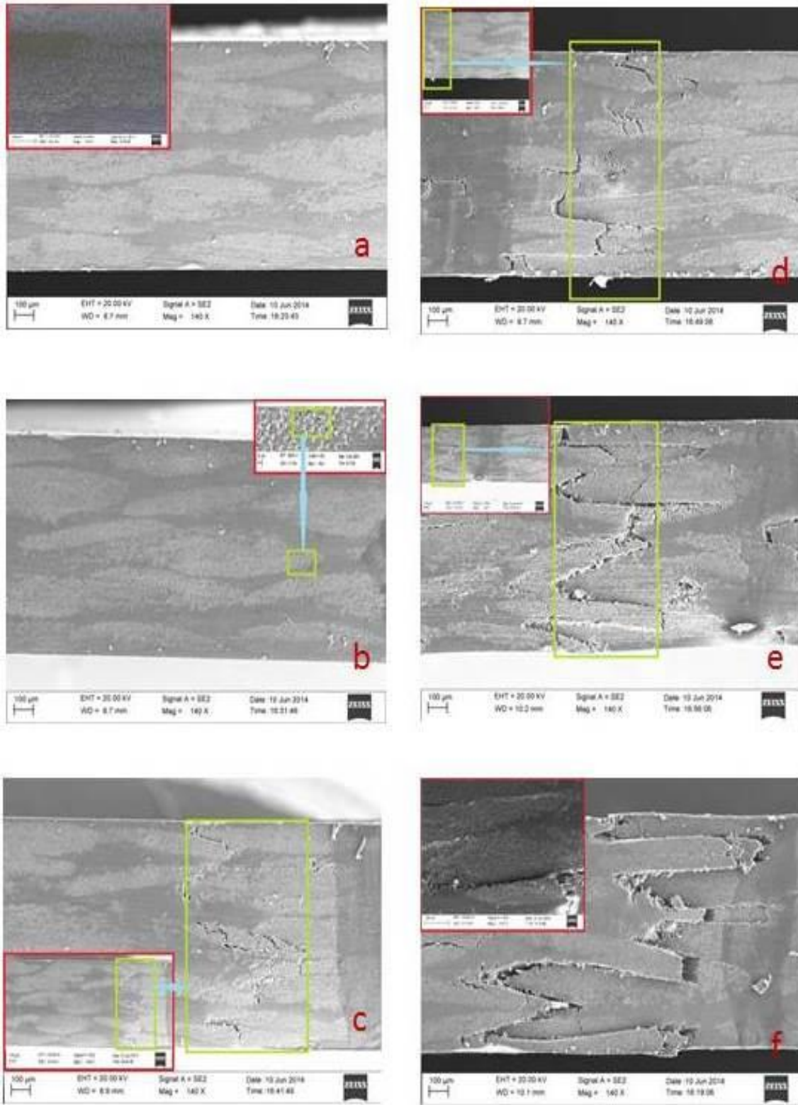
Figure 6.17 SEM images (a) undamaged, (b) 2 kN, (c) 2.5 kN, (d) 3 kN, (e) 3.2 kN (f) failed.
