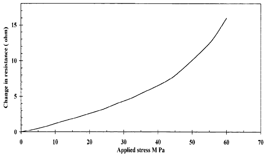
Figure 2.9: Change in resistance for 90° samples [83].
