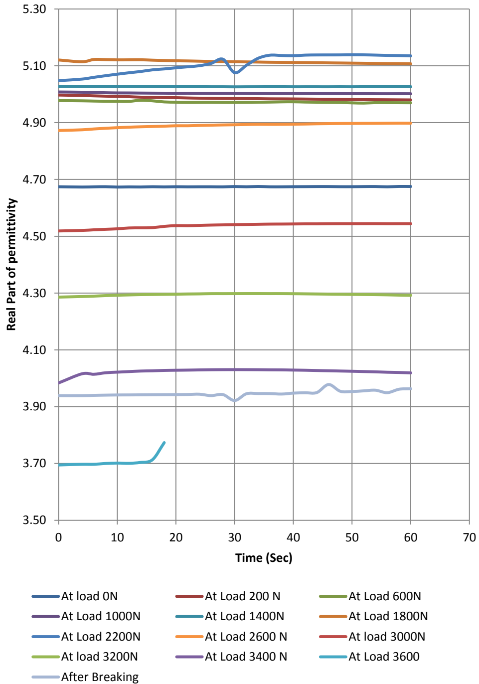
Real part of Permittivity Vs Time in different Load
