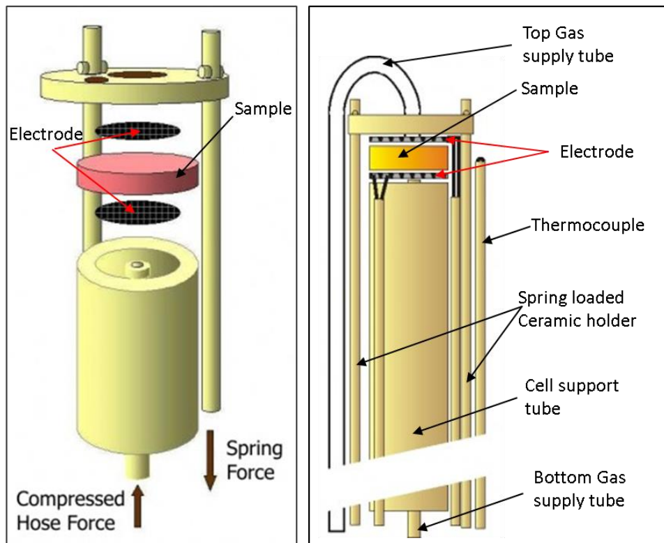
Figure 3.4 Probostat™ spring loads and regular 2-electrode 4-wire setup with dual gas supplies and thermocouple
