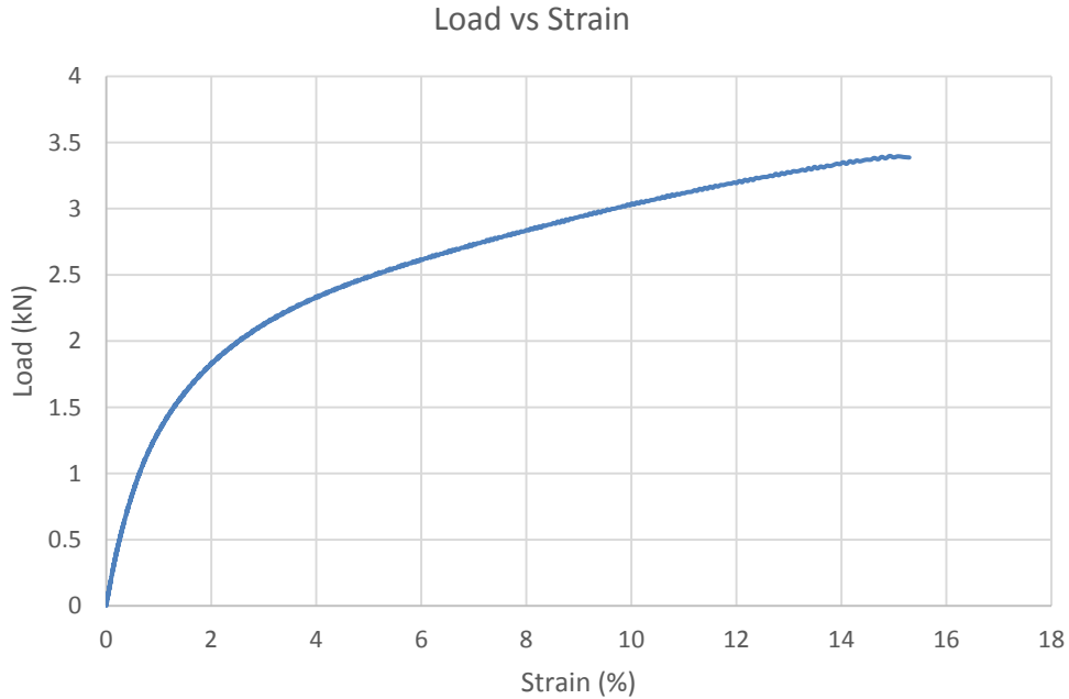
Figure 6.5 Load-strain curve
