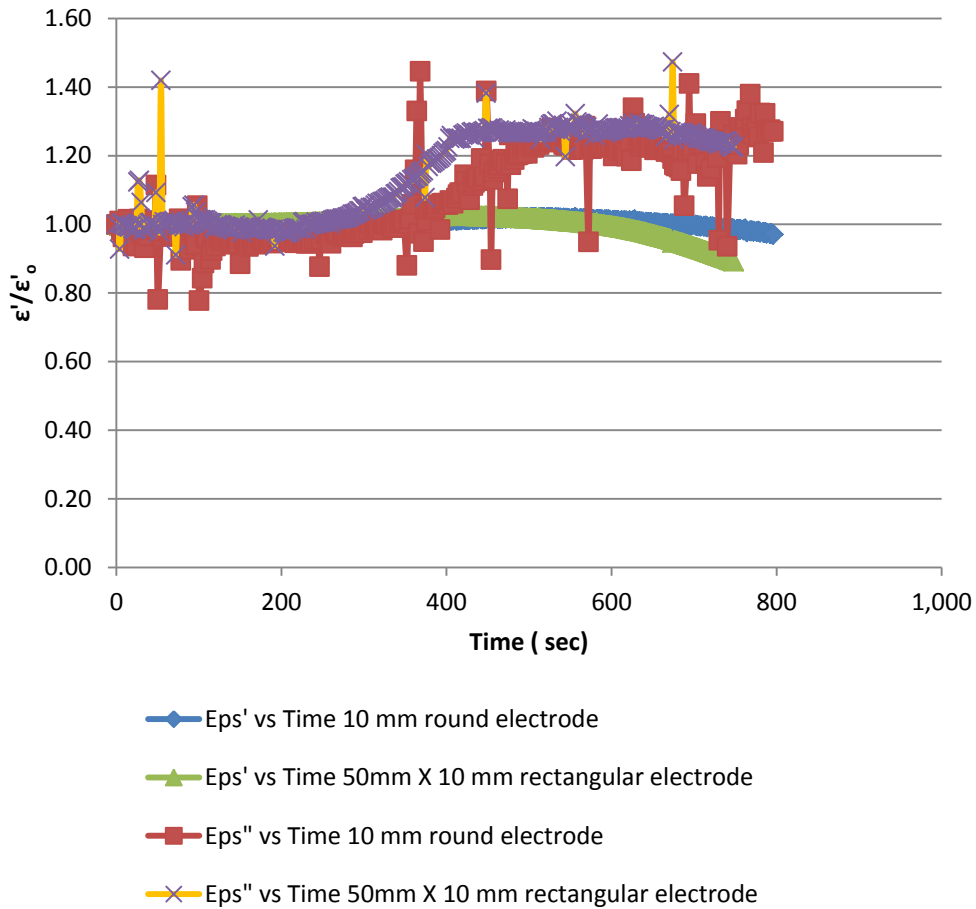
Figure 5.10 Comparison of the dielectric properties for different electrode arrangement.
