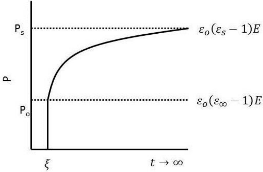
Figure 2.12 Time dependence of polarization, P , when a constant electric field is applied at t = \xi
