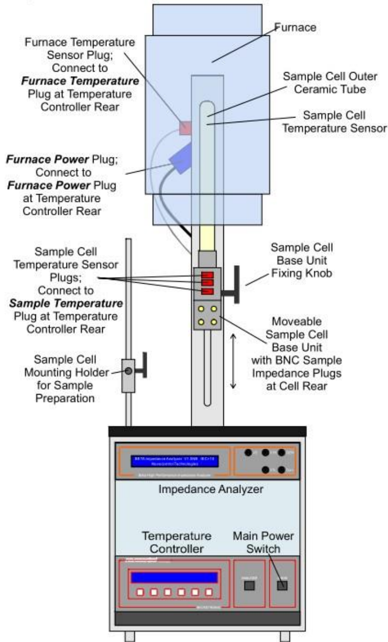
Figure 3.1 Novocontrol™ system
