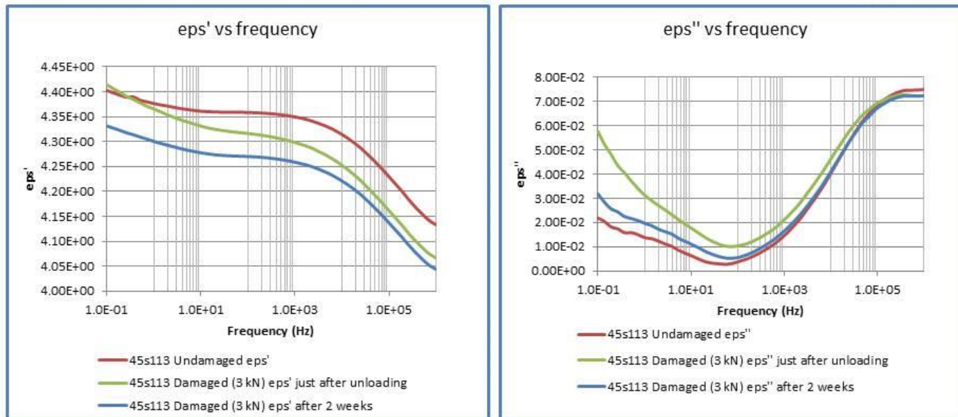
Figure 6.13 Mechanical and dielectric properties of the sample 45s113
