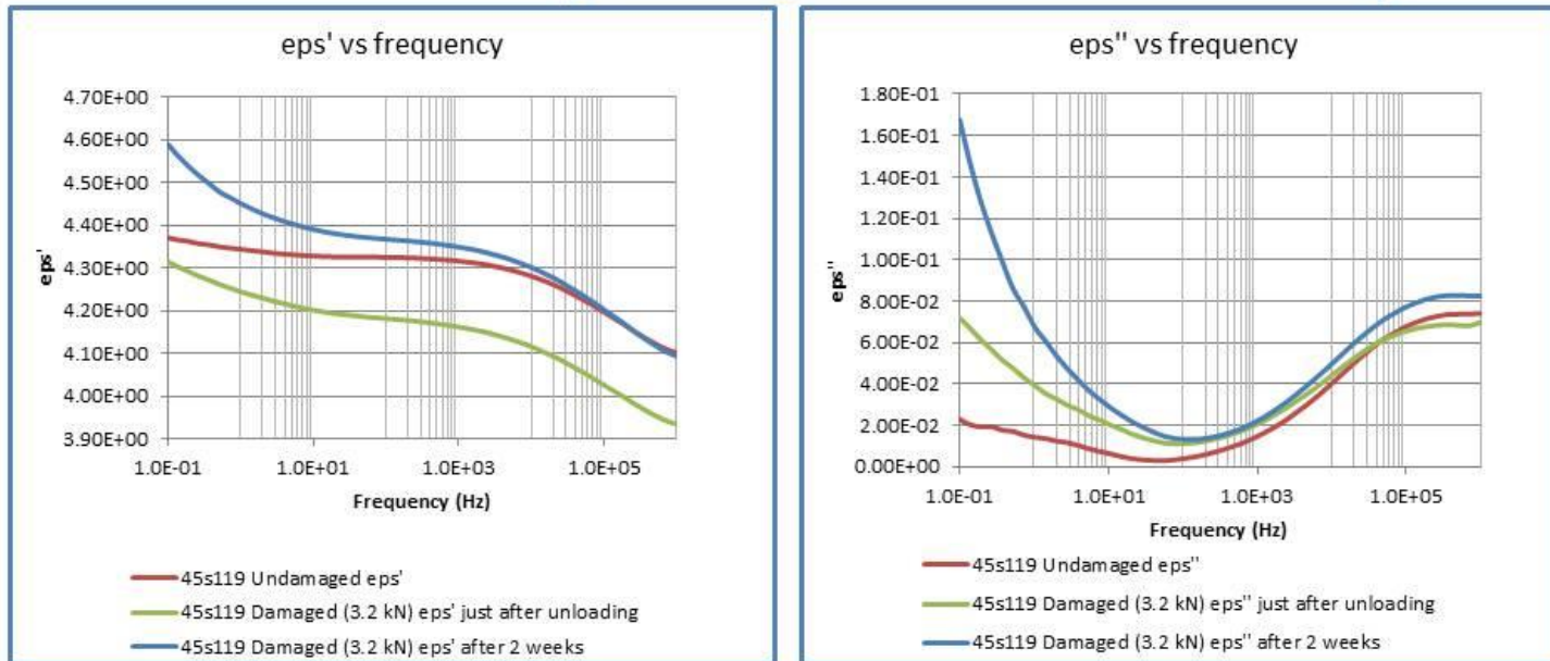
Figure 6.16 Mechanical and dielectric properties of the sample 45s119
