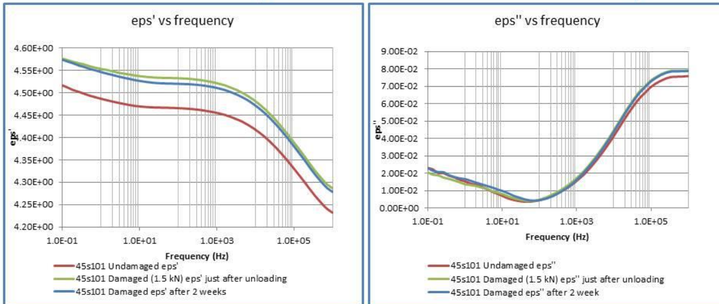
Figure 6.7 Mechanical and dielectric properties of the sample 45s101
